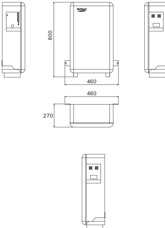
Fig. 5-1 Product Dimensions
