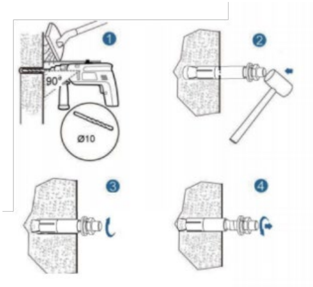
Fig.6-2 Fix the Battery to the Wall
