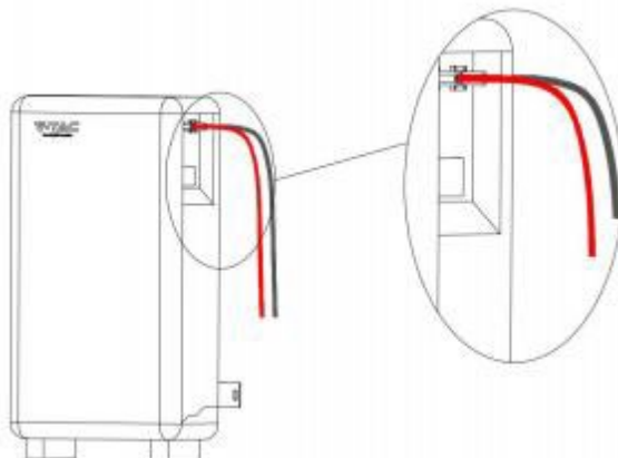
Fig.6-4 Power Cable Connection Diagram
