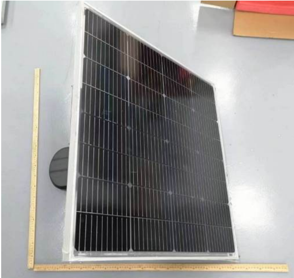
Overall view for FC-60W
