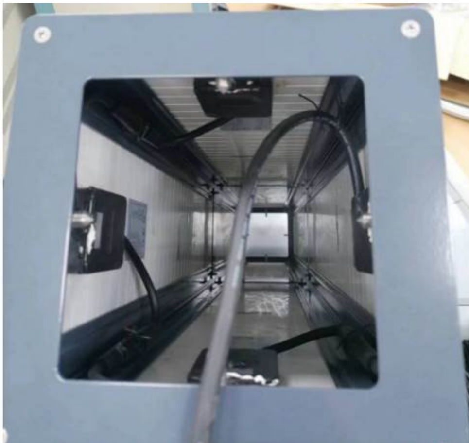
Internal view of solar panel for W-100
