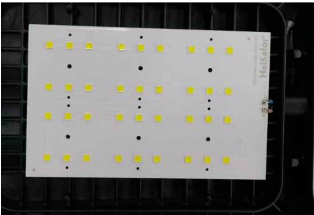
LED module view for FC-60W
