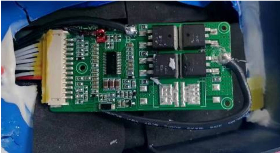
PCB of battery protection board view for W-100 and FC-120
