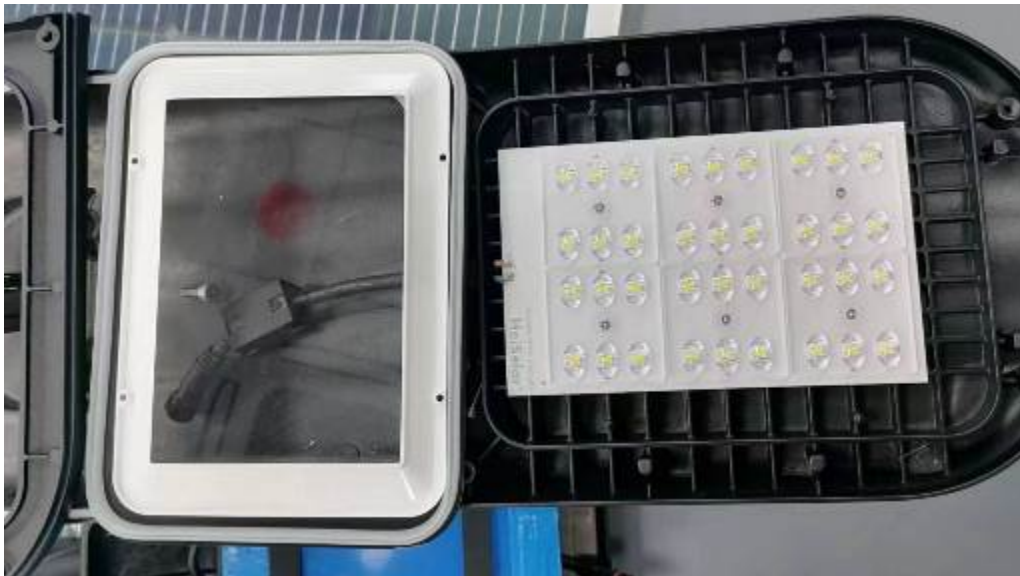
LED lens view for FC-60W
