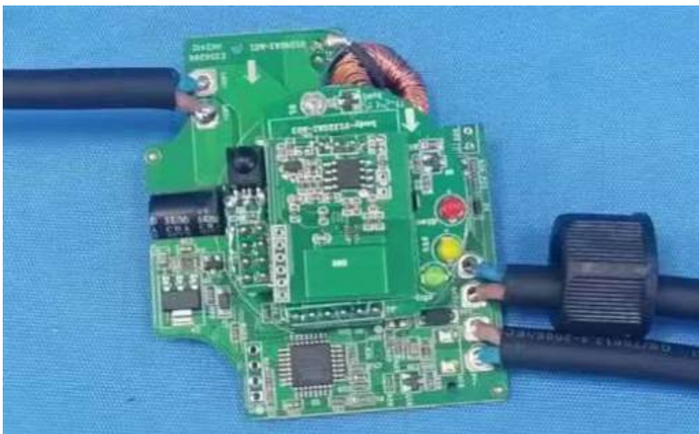
PCB view of control device for FC-60W
