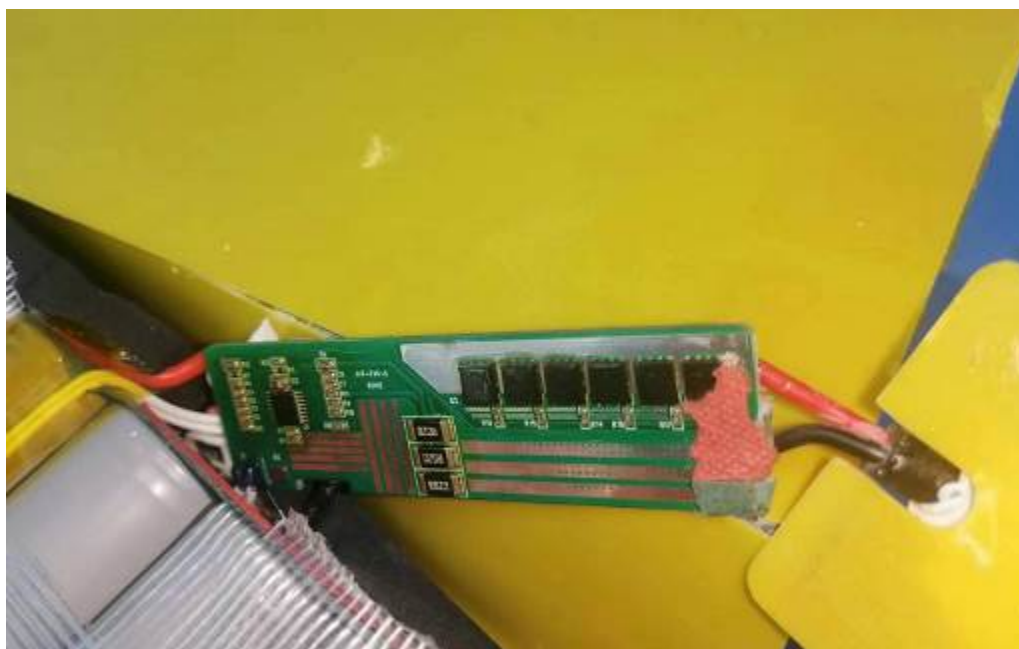
Battery protection board view for FC-60W
