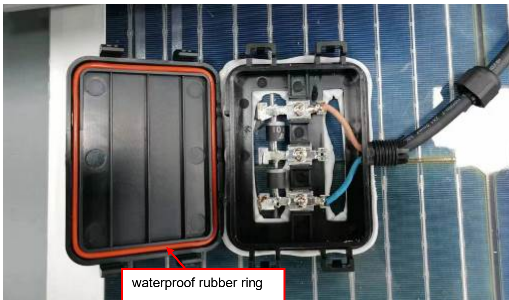
Solar connecting box view for FC-60W
