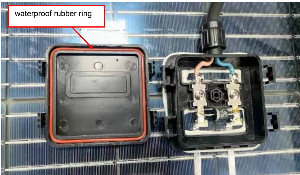
Lead wire of solar panel view for FC-120
