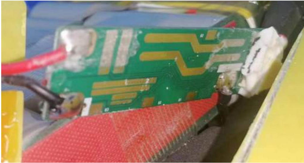
Battery protection board view for FC-60W
