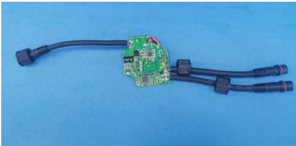
Internal of control device without enclosure view for FC-60W
