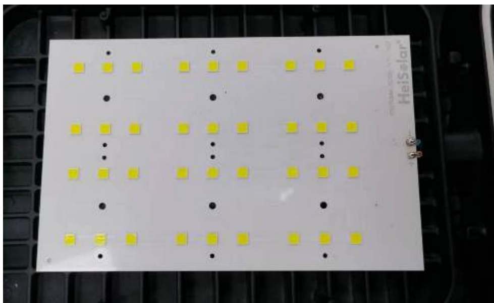
LED module view for FC-120
