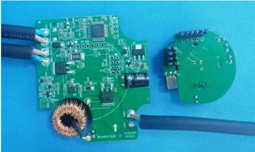
Explosive view of control device PCB for FC-60W
